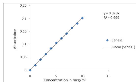
Figure 1. Standard Calibration Curve of Balofloxacin
