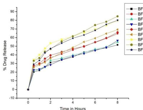
Figure 2. Dissolution of Balofloxacin floating tablets Batches BF1 to BF9
