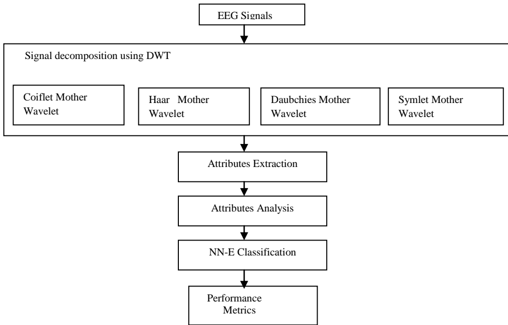
Fig 1: The proposed methodology for classification of EEG signals
