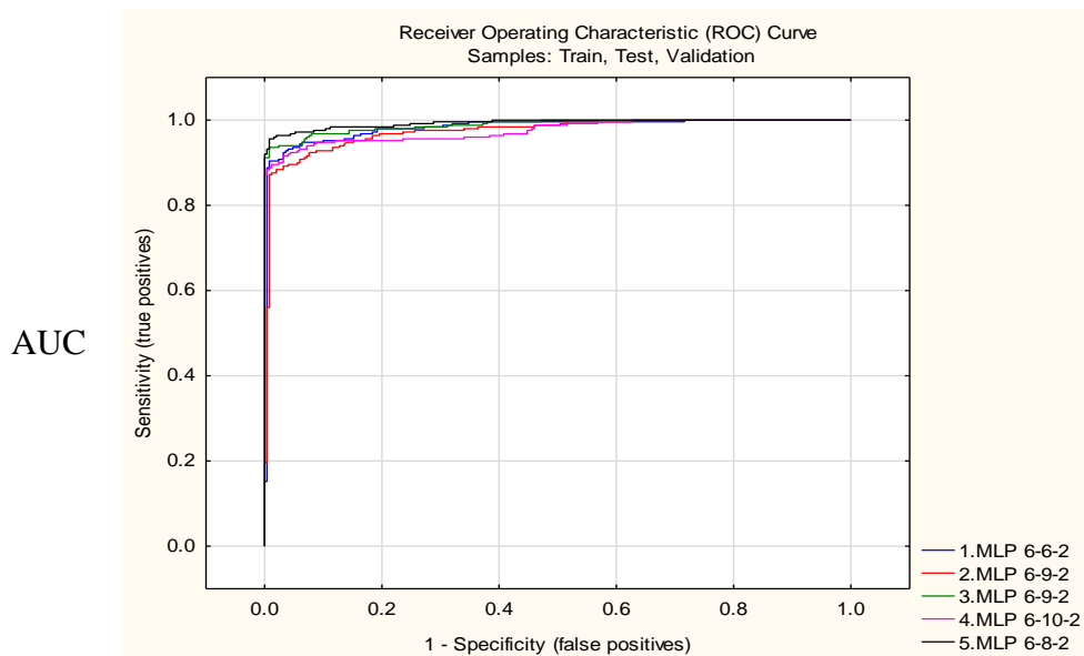
Fig 4: ROC curves for different configurations of NN-DB ensemble
